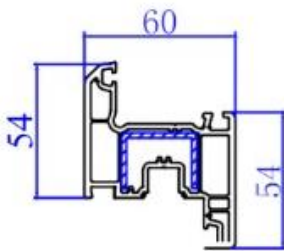
60 Inward Window Sash 410200
