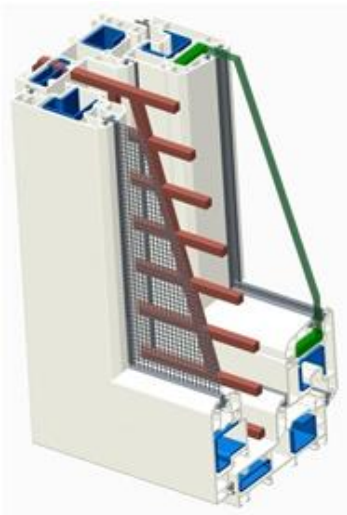
Double Rebate (Double PATAM) Villa Windows Section
