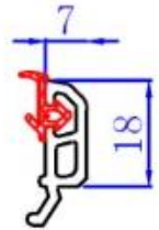
88 Sliding Sash 411000
