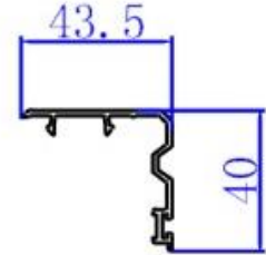
Cover Profile for Sliding Door 421100
