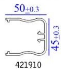
Hurricane Bar
