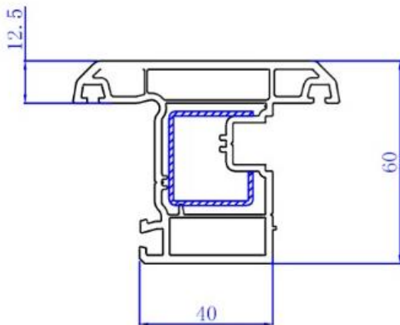
60 Outward Window Sash 410300
