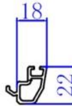
Glazing Bead 22 421200
