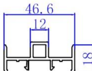
Interseal 421000
