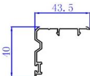
Cover Profile 421100
