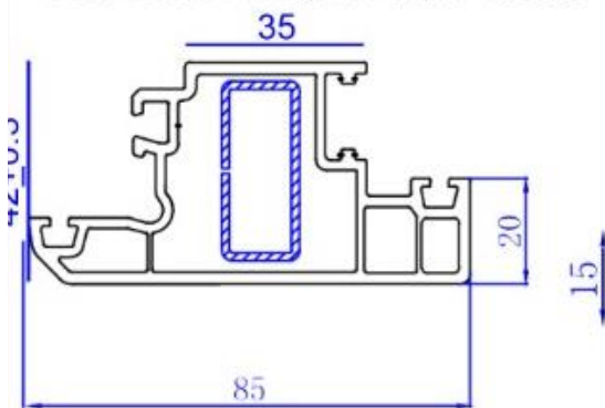
Villa Window Mosquito Sash 430020
