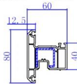
60 Outward Window Sash 410300
