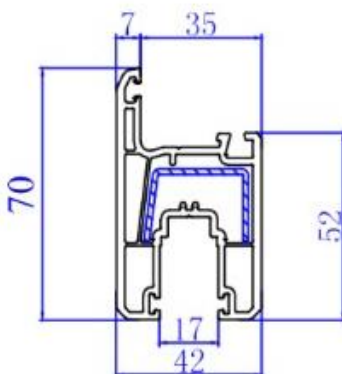
88 Sliding Sash 411000
