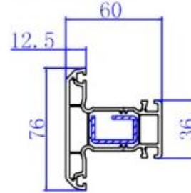
60 Window Mullion 410400
