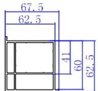
60 Square Post 420500
