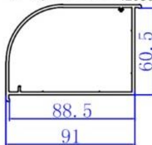
88 Square Post 420800
