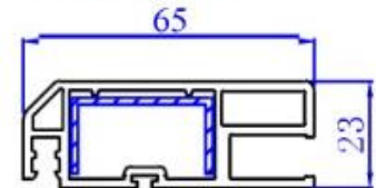
88 Mosquito Sash 421900
