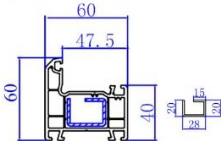
60 Window Frame 410100
