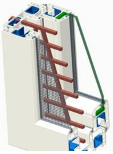
Villa Window Mosquito Sash 430020
