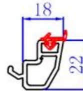
Glazing Bead 22 421200
