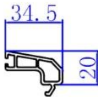
Glazing Bead 34.5 420200
