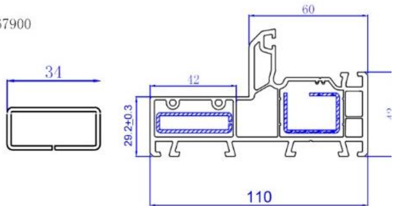
430010 Villa Window Outer
