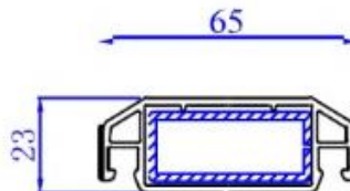
88 Mosquito Sash Mullion 421700
