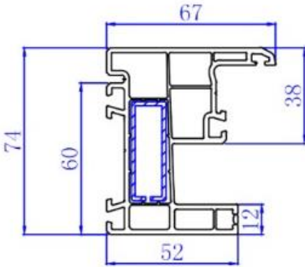
Mono Rail Outer 412200
