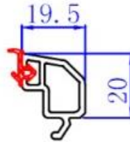
Mono Rail Mullion 412400
