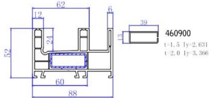
88 Sliding Mullion 411700
