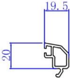
Glazing Bead 19.5 420100
