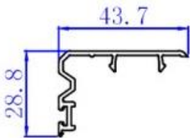
Cover Profile 420700
