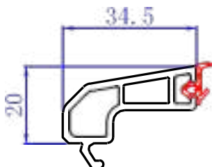
GLAZING BEAD 34.5 320400
