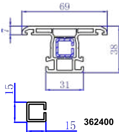
MONORAIL MULLION 312400
