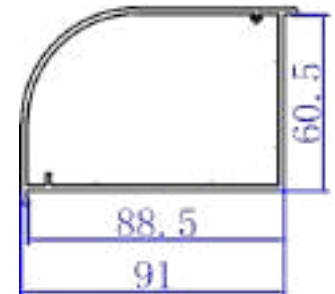
88 SQUARE POST 320800
