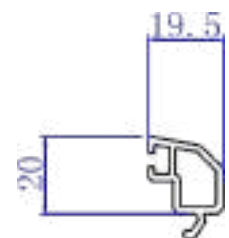
GLAZING BEAD 19.5 320100
