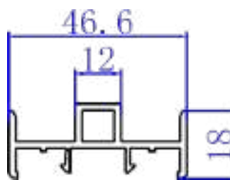
INTERSEAL 321000
