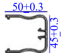
HURRICANE BAR 321910
