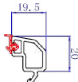
GLAZING BEAD 19.5 320100
