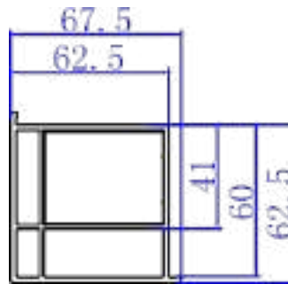
60 SQUARE POST 320500
